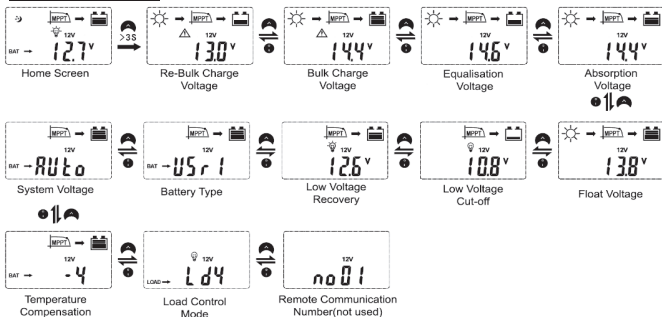
Figure 8 Settings Flow Chart
