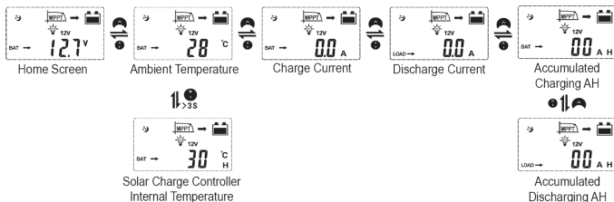
Figure 7 Main Navigation Flow Chart
