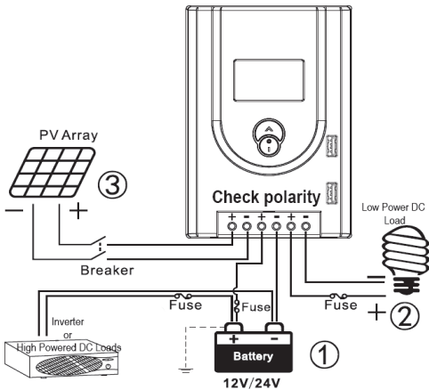
Figure 3 Connection Diagram
