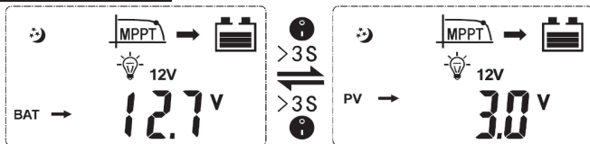
Figure 14 Solar Input Voltage
