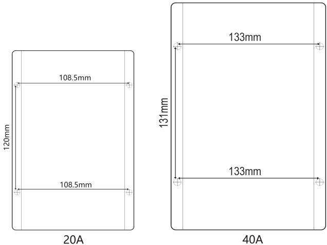
Figure 2 Mounting Diagram
