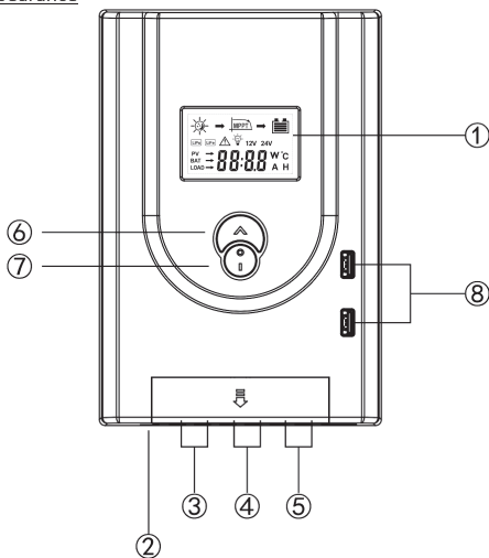
Figure 1 Solar Controller Features
