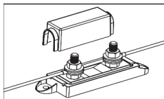
Figure 4 Bolt Down Fuse Holder
