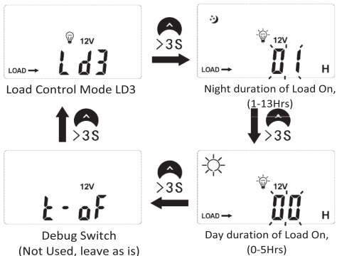
Figure 13 Dual Time Mode Flow Chart
