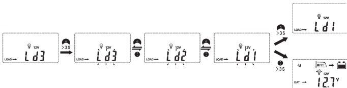
Figure 9 Changing Parameters
