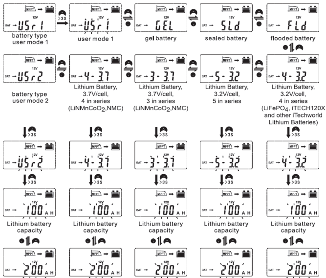
Figure 10 Battery Selection Flow Chart
